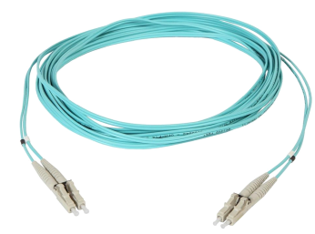
Fiber Optic Patch Cord, OM4, LC duplex to LC duplex, 1.8 mm LSZH, 6 m, aqua
