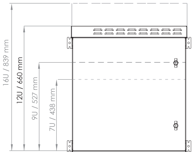
CABINET HEIGHTS
