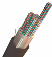
250µm Wrapping Tube Cable (WTC) with SpiderWeb Ribbon® (SWR®)
